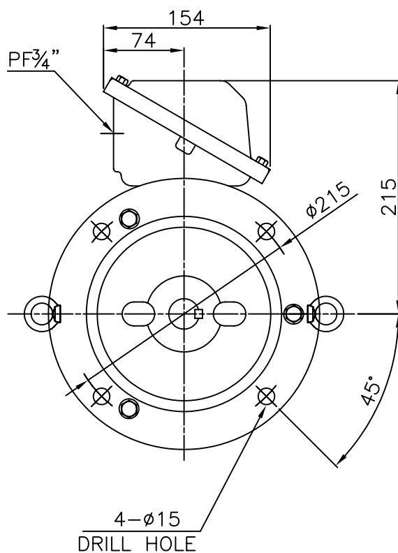
VIEW "A"
