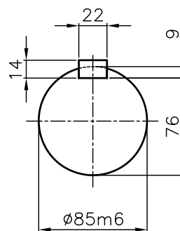
VIEW "A"
