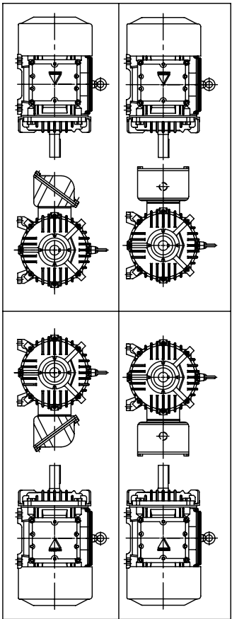
* TERMINAL BOX LOCATION
