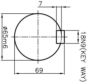
VIEW "A" SCALE 2.5/1
